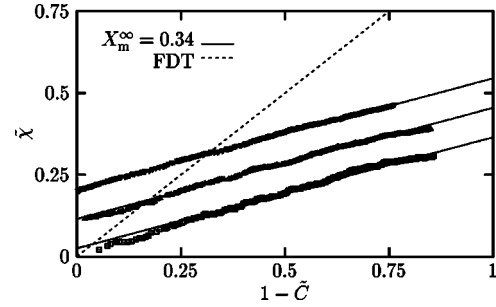
FIG. 1. Normalized FD plot for magnetization in the d=2 Ising model at T_c for times t_w=46, 193, and 720 (bottom to top). Curves have been vertically shifted by 0, 0.1, and 0.2 for clarity. The convergence for large t_w to an almost straight line of slope X^\infty \approx 0.34 is evident.
